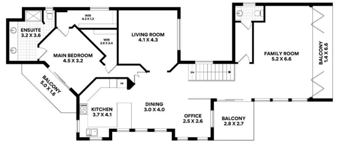
THIRD FLOOR
